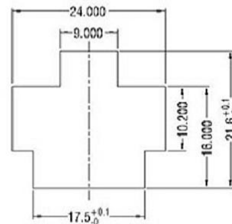
PANEL CUT-OUT
